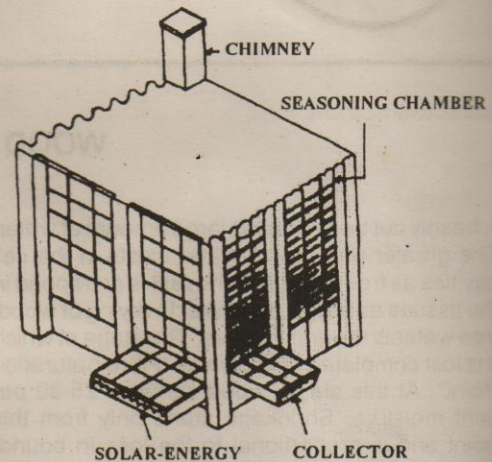
Fig. 2 : Solar Timber Seasoning Kiln
