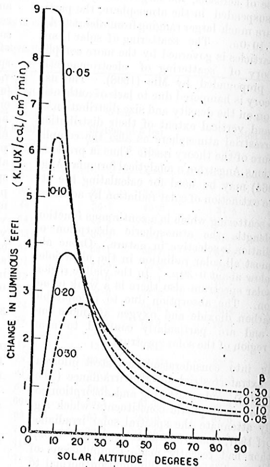
Fig. 1. Change in luminous efficiency of direct solar radiation at an altitude of 5000 m over that at m.s.l.
