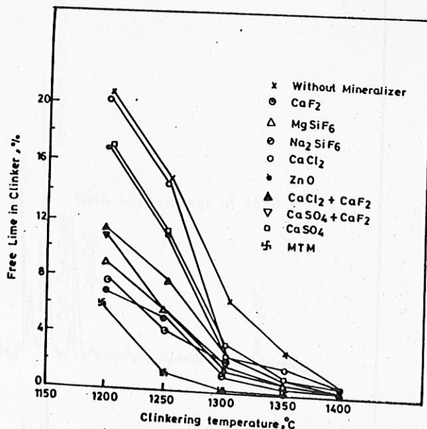
Fig. 1—Effect of clinkering temperature on lime fixation
