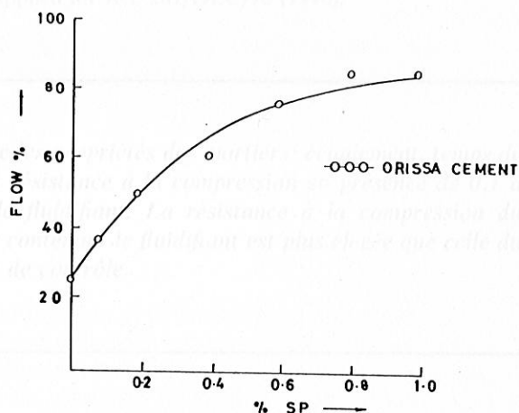
Fig. 2 Effect of superplasticizer dosage on flow properties of mortar at 0.45 w/c ratio (Orissa cement).
