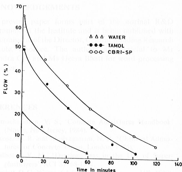
Fig. 1 Variation of flow of 1:3 cement:sand mortar (at 0.45 w/c ratio) with time.
